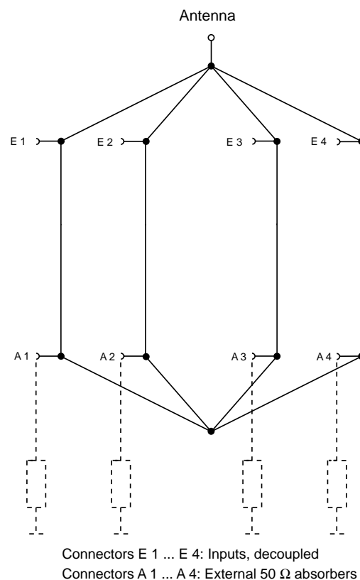
1:4 power splitter 725 234
